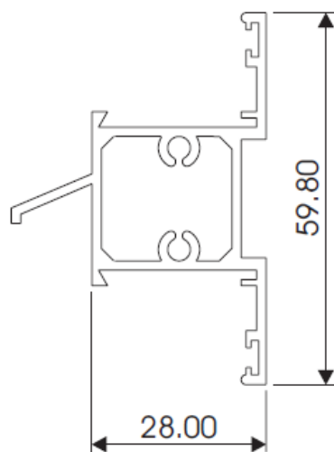
28mm WEATHER BAR MULLION AL851
