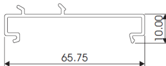
SIDELIGHT ADAPTOR AL850
