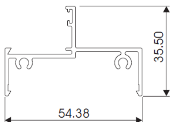
54mm FRAME AL850
