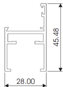
28mm EQUAL LEG AL057
