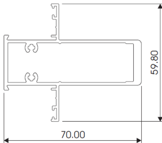
70mm MULLION AL557
