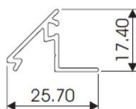
4mm BEAD AL060
