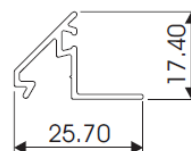
MULTI BEAD AL555
