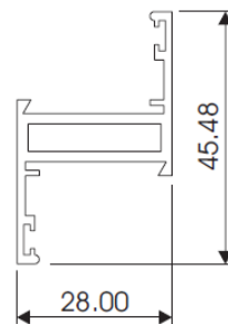
28mm SASH AL058
