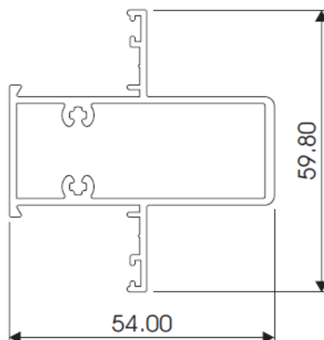
54mm MULLION AL556
