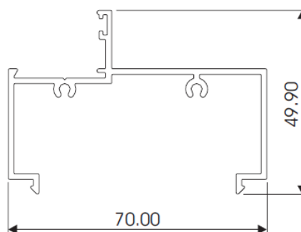
70mm FRAME AL554
