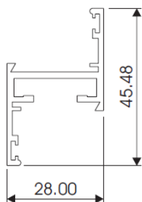
28mm UNEQUAL LEG AL371
