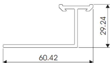
TWIST IN FIXING LUG AL064
