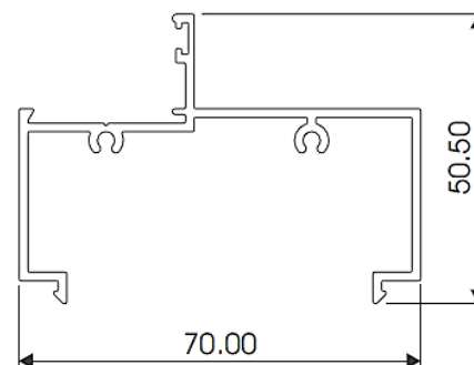
70mm FRAME
