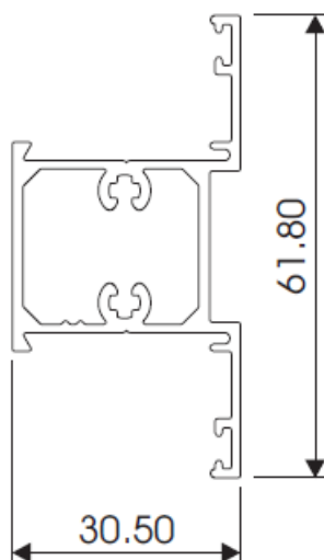
30.5mm MULLION AL488
