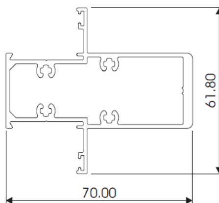
70mm MULLION AL747
