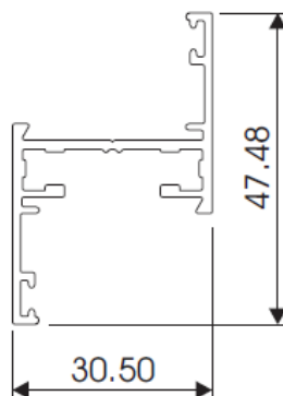
30.5mm UNEQUAL LEG
