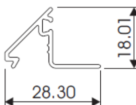
MULTI BEAD AL489
