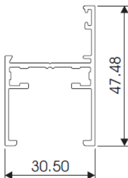
30.5mm EQUAL LEG AL486
