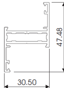
30.5mm SASH AL487
