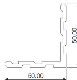
50mm CORNER CLEAT AL062
