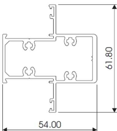
54mm MULLION AL746
