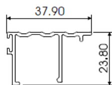
THRESHOLD COVER AL614
