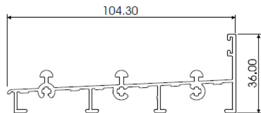
TRIPLE FRAME SILL AL626
