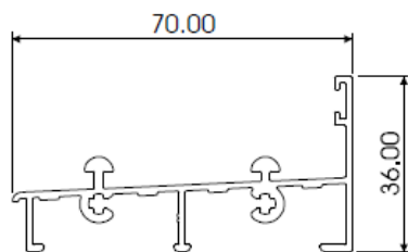
FRAME SILL AL613
