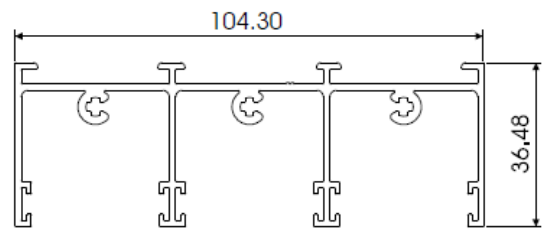
TRIPLE FRAME HEAD AL625
