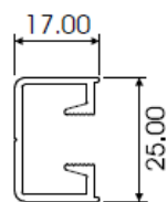
FIXED STILE AL621
