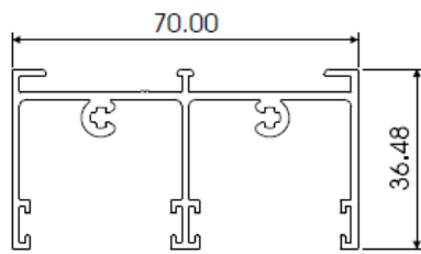
FRAME HEAD AL611
