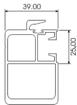
EXTRA H/DUTY INTERLOCK AL629
