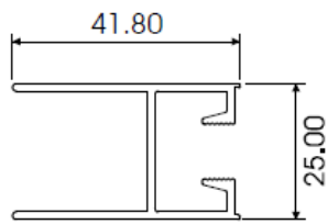
FIXED STILE AL622
