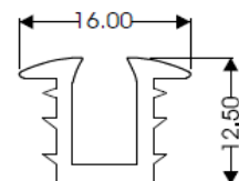
CHANNEL GASKET
