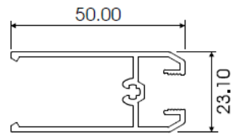
SASH HEAD AND SILL RAIL AL616
