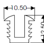
CHANNEL GASKET
