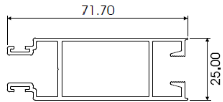
OXO MALE MEETING STILE AL623
