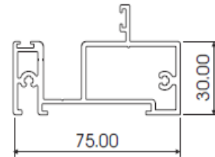
VISTAFOLD HEAD AL561
