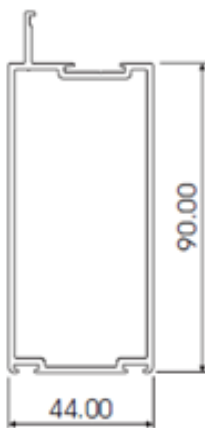
K90mm D/STILE W/PILE AL026
