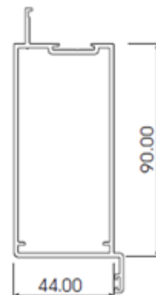
KR12 90mm D/STILE AL350
