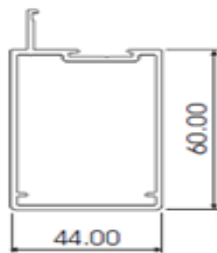
KR60mm D/STILE AL024
