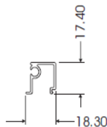
KSQ BEAD AL013
