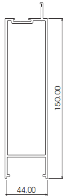
KR6 BOTTOM RAIL AL010
