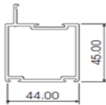
KR3 AL007
