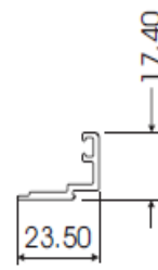
DOUBLE GLAZE BEAD AL360
