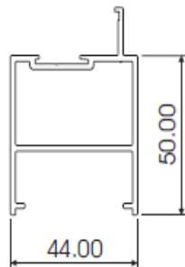
KR7 TOP RAIL AL011
