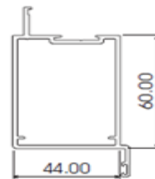
KR12 60mm D/STILE AL350
