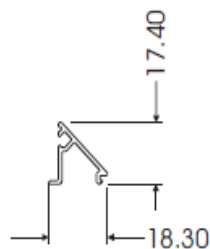
K45 BEAD AL012
