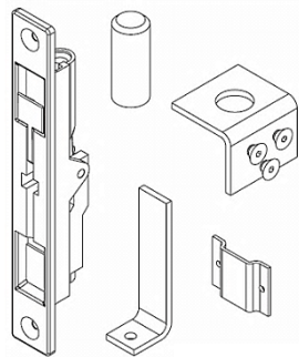
DOUBLE ACTION FLUSH BOLT
