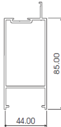
KR4 BOTTOM RAIL AL005
