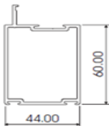
KR60mm D/STILE W/PILE AL550
