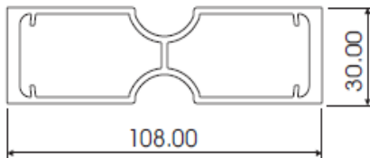
VISTAFOLD HEAVY DUTY MULLION AL743
