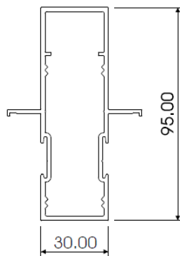
K95 2 LIP AL379
