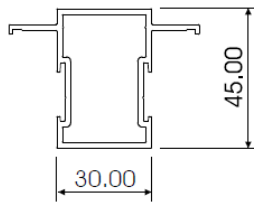
GLAZING BAR AL014
