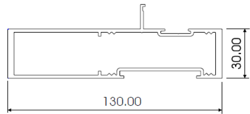
K130B RECESSED BACK AL855
