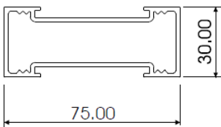
K26D RECESSED BACK AL454
