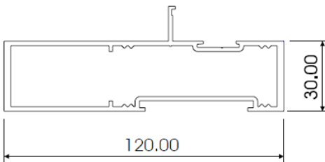
K120B RECESSED BACK AL854
