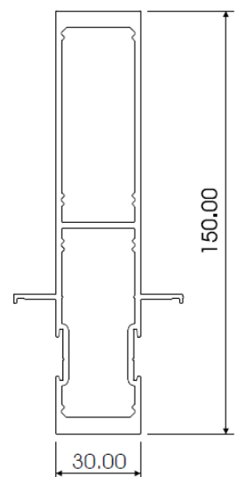
K150 2 LIP HEAVY DUTY AL858
