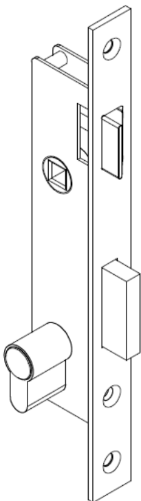
25/35mm BACKSET LATCH LOCK
