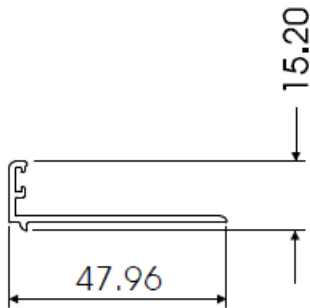
ASTRAGAL WITH WOOLPILE AL009
