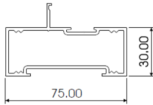
K26B RECESSED BACK AL001
