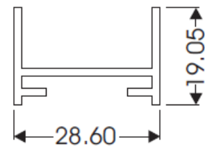
"Y" LOUVRE FRAME AL153
