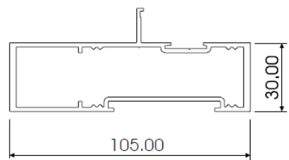
K105B RECESSED BACK AL551
