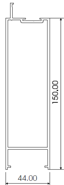
KR6 BOTTOM RAIL AL010
