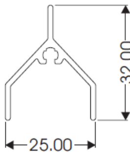
"Y" LOUVRE AL152
