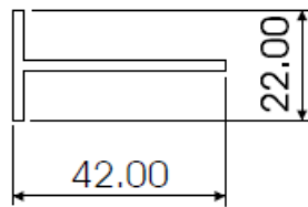
NO.12 ASTRAGAL TEE AL045
