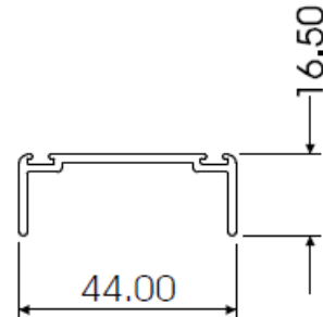
PIVOT DOOR HEAD ADAPTOR AL361
