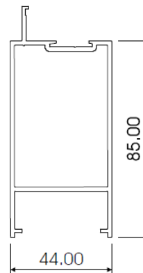
KR4 BOTTOM RAIL AL005
