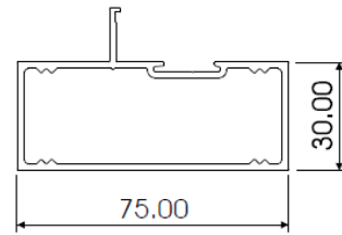
K26B FLAT BACK AL434
