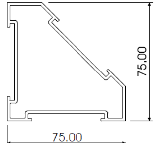
CORNER MULLION AL018
