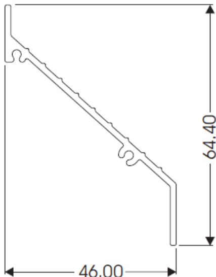
LAZY "Z" LOUVRE AL155
