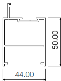
KR7 TOP RAIL AL011
