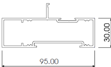
K95B RECESSED BACK AL853
