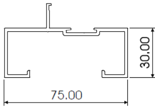
K26C OPEN BACK AL003
