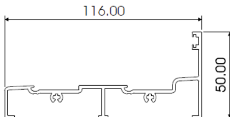
DOUBLE SILL AL364
