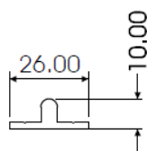
FLOOR TRACK AL216
