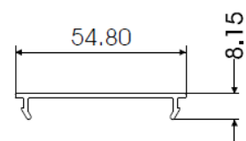
DOUBLE HEAD COVER AL365
