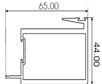
INTERLOCK FIXED 65mm AL720
