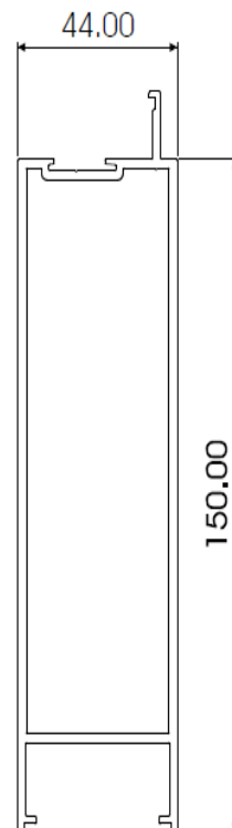
KR6 BOTTOM RAIL AL005
