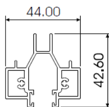
SILL EXTENTION AL609
