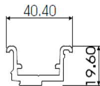
R4 SPIGOT SECTION AL028
