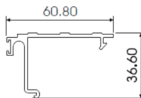
SILL COVER AL368
