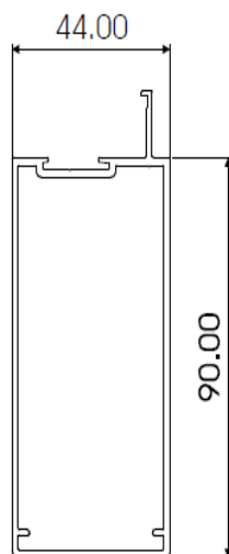
K90mm D/STILE AL025
