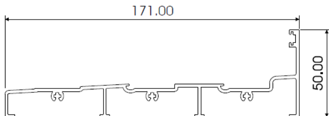
TRIPLE SILL RAIL AL633
