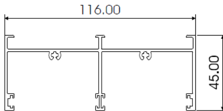
DOUBLE HEAD RAIL AL363
