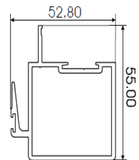
INTERLOCK SLIDE 40mm AL022
