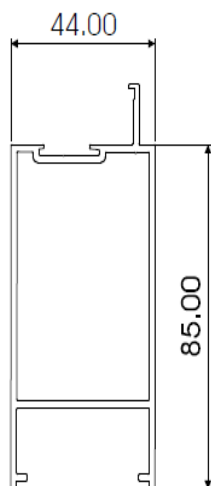
KR4 BOTTOM RAIL AL005
