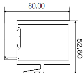
INTERLOCK SLIDE 65mm AL722
