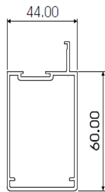
KR60mm D/STILE AL024
