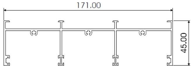
TRIPLE HEAD RAIL AL632
